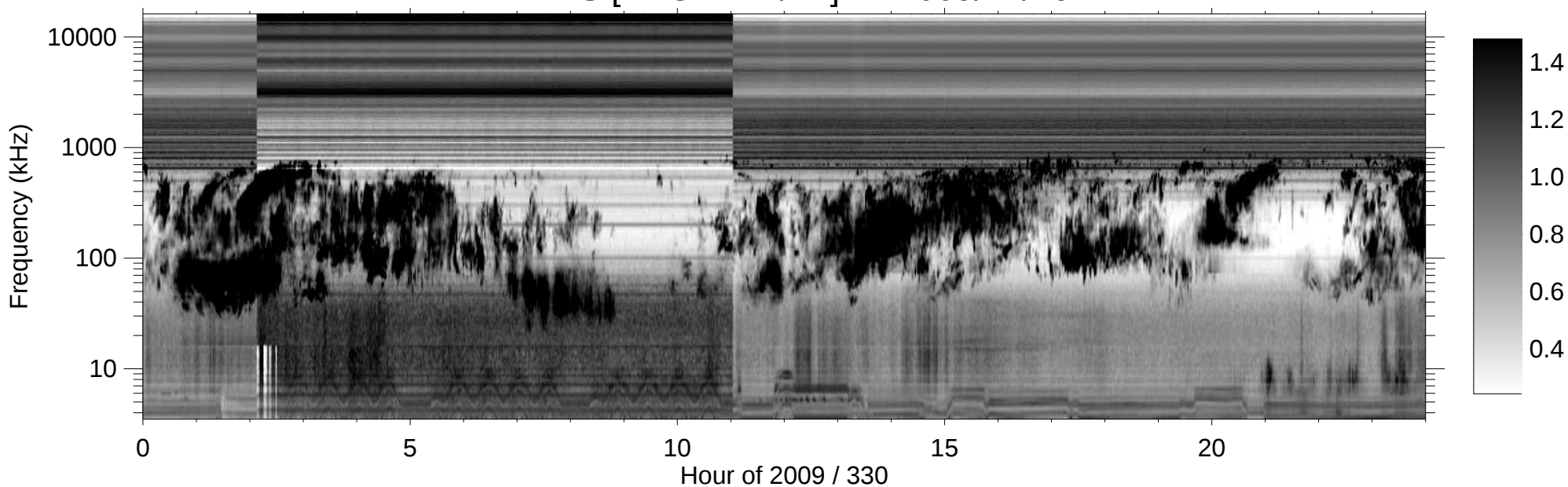
RPWS [ABCH1H2/Ex] (-B) 2009/11/26
