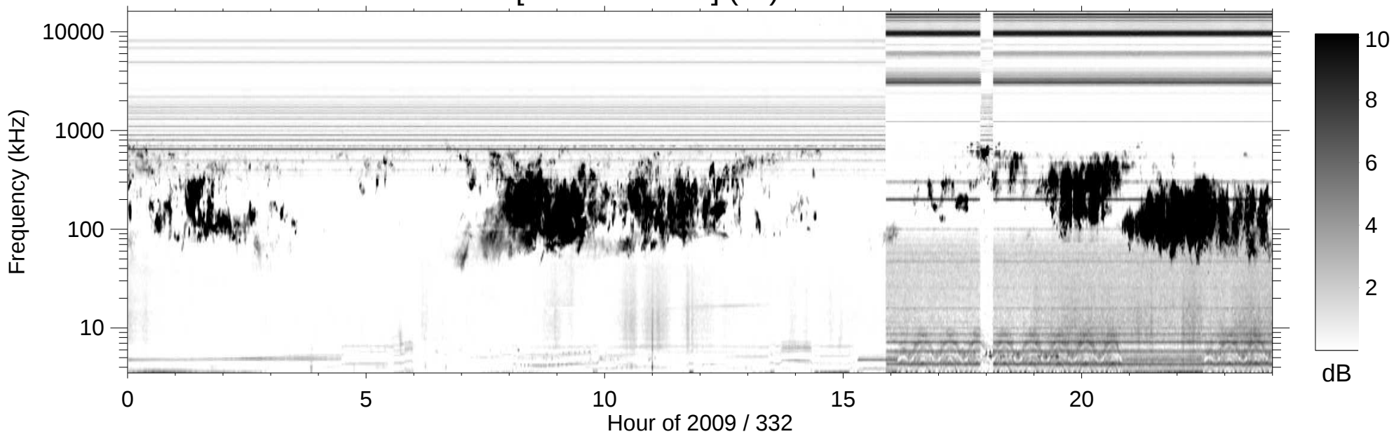
RPWS [ABCH1H2/Ex] (-B) 2009/11/28
