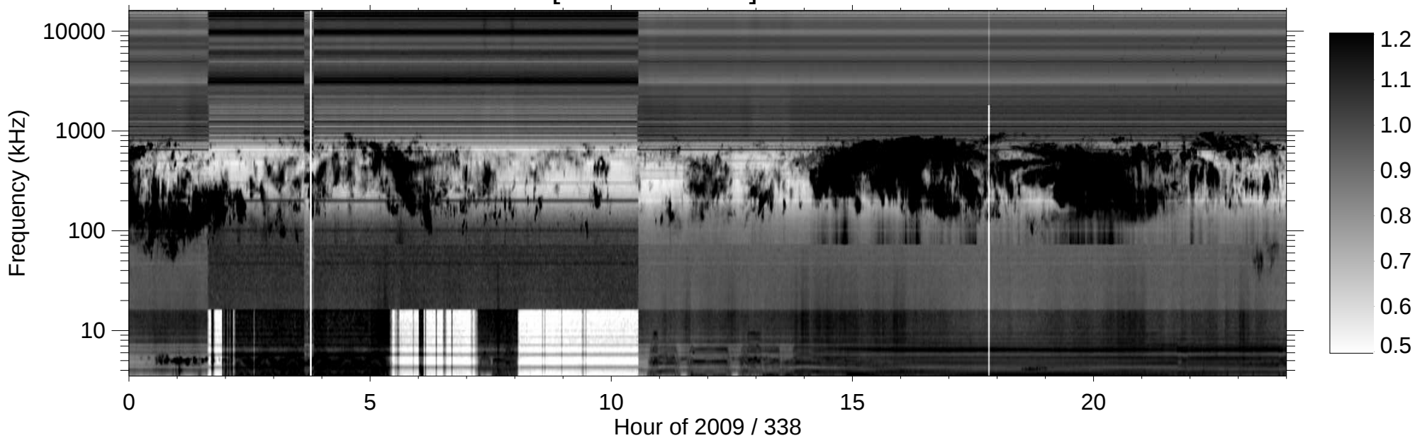
RPWS [ABCH1H2/Ex] (-B) 2009/12/04
