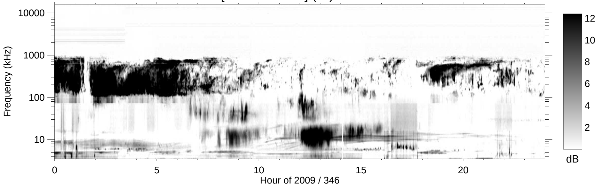
RPWS [ABCH1H2/Ex] (-B) 2009/12/12
