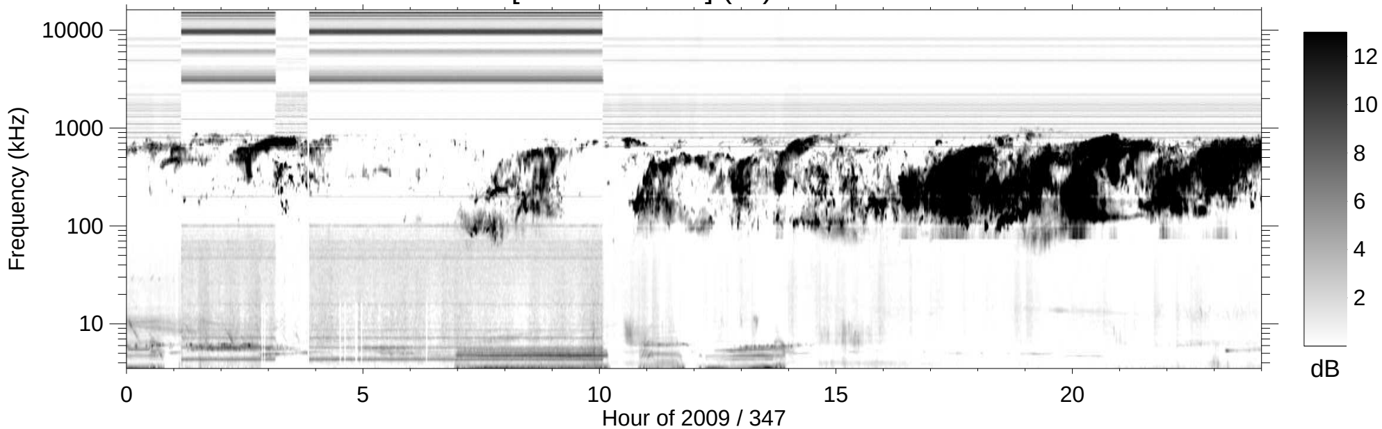
RPWS [ABCH1H2/Ex] (-B) 2009/12/13
