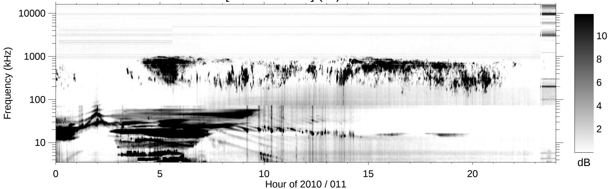
RPWS [ABCH1H2/Ex] (-B) 2010/01/11
