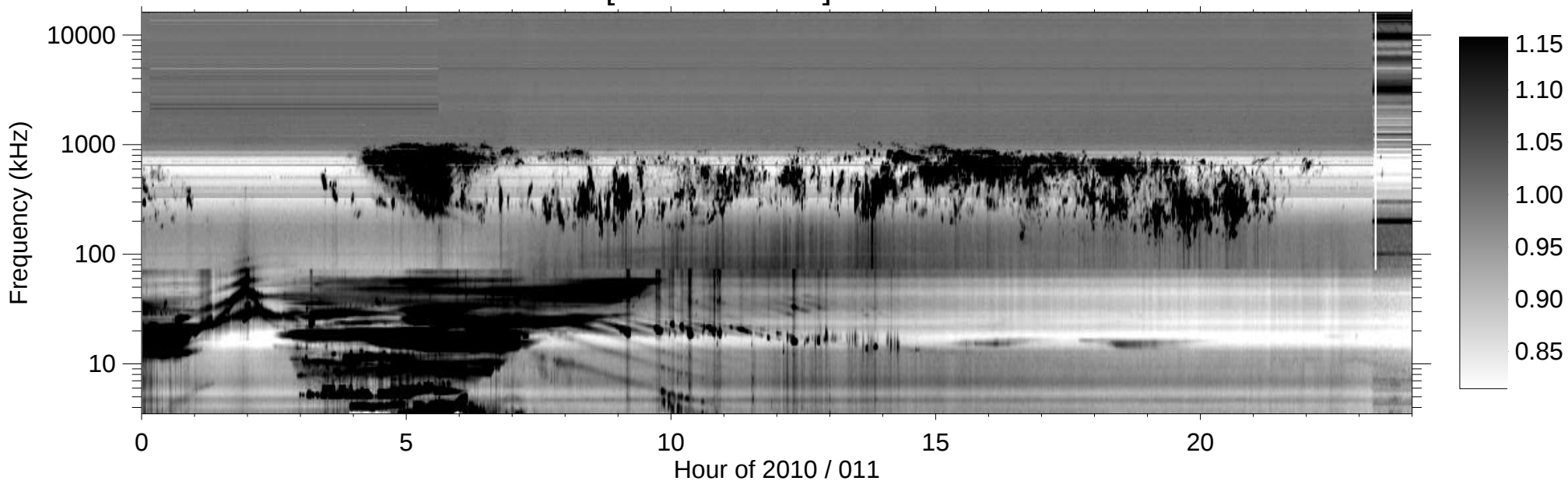
RPWS [ABCH1H2/Ex] (-B) 2010/01/11
