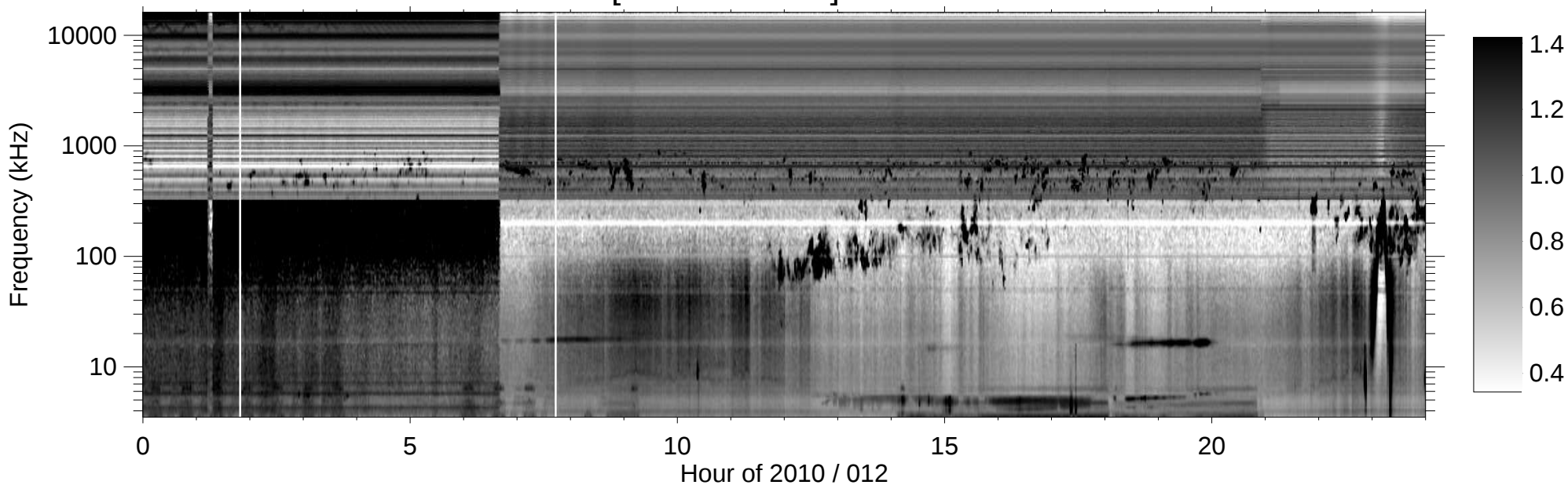
RPWS [ABCH1H2/Ex] (-B) 2010/01/12
