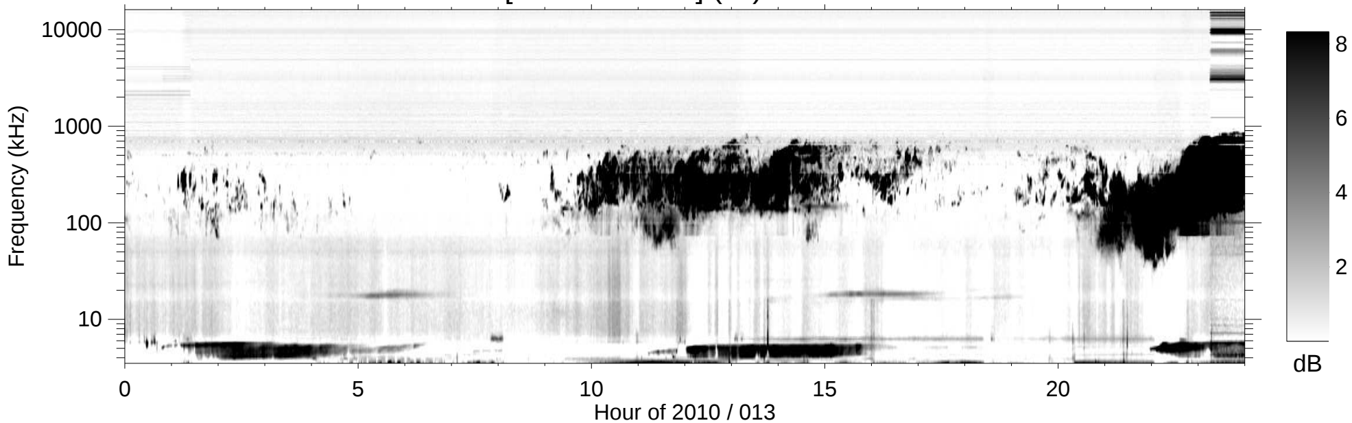
RPWS [ABCH1H2/Ex] (-B) 2010/01/13
