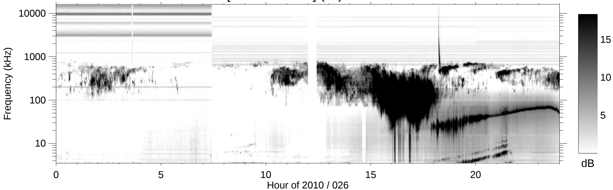
RPWS [ABCH1H2/Ex] (-B) 2010/01/26
