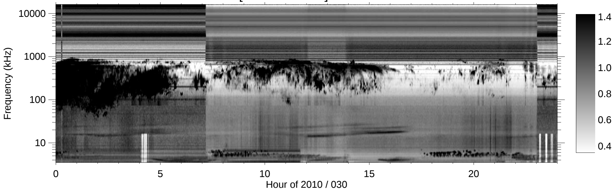
RPWS [ABCH1H2/Ex] (-B) 2010/01/30
