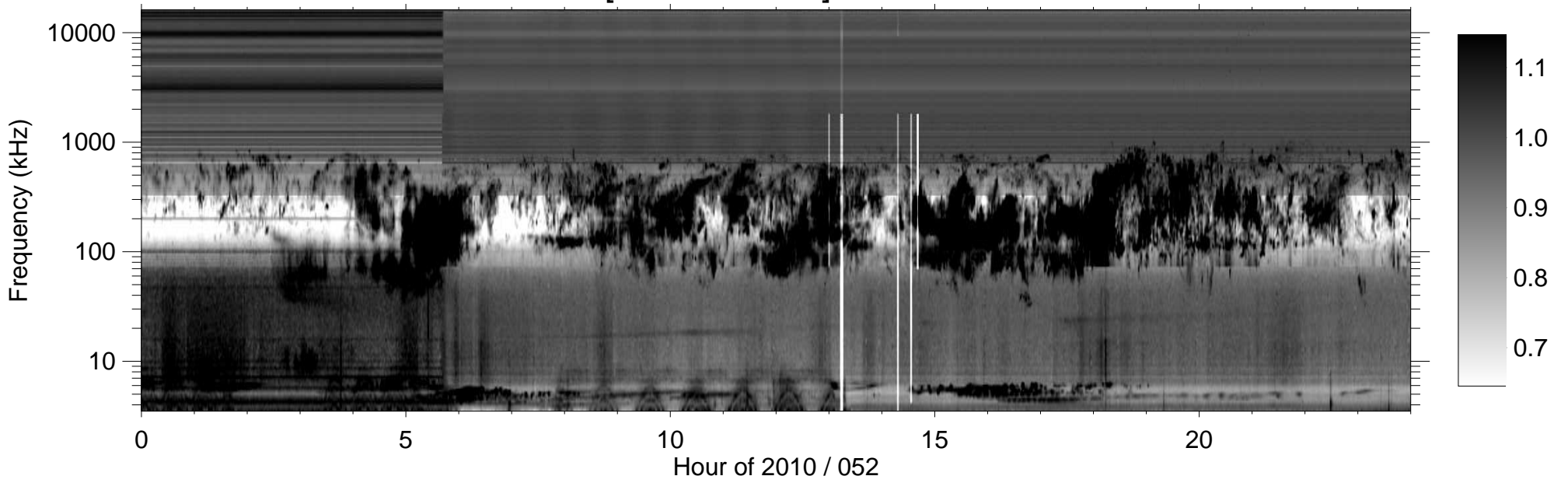
RPWS [ABCH1H2/Ex] (-B) 2010/02/21
