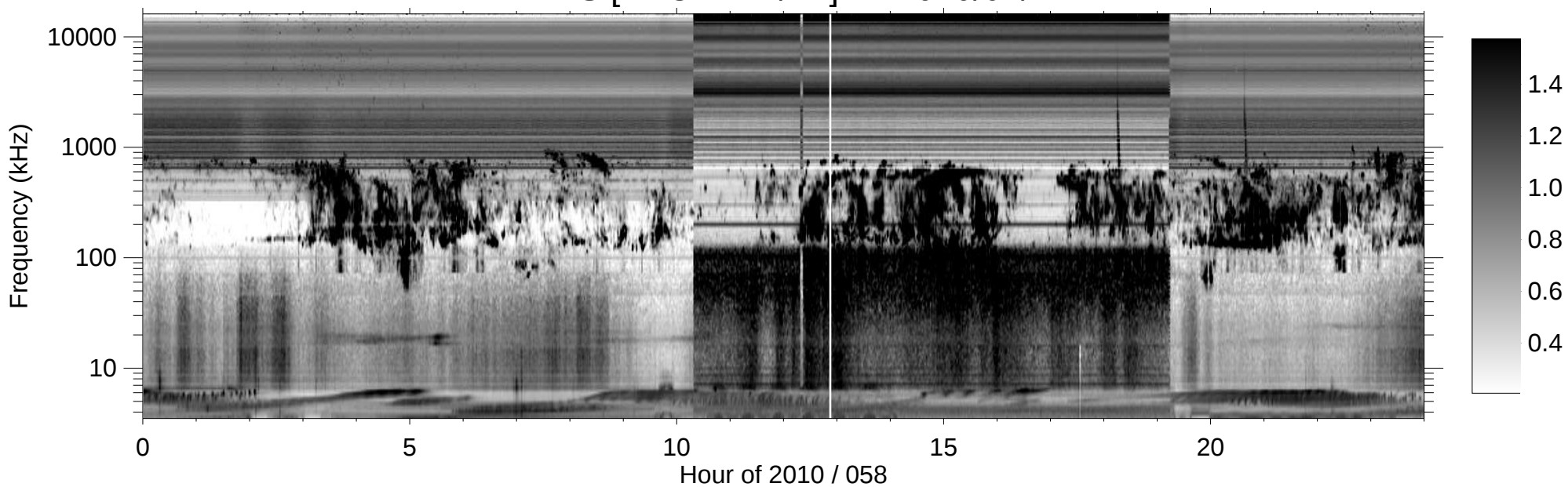
RPWS [ABCH1H2/Ex] (-B) 2010/02/27
