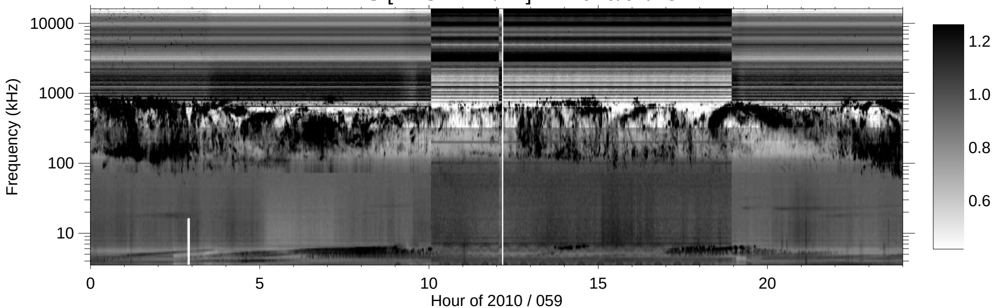
RPWS [ABCH1H2/Ex] (-B) 2010/02/28
