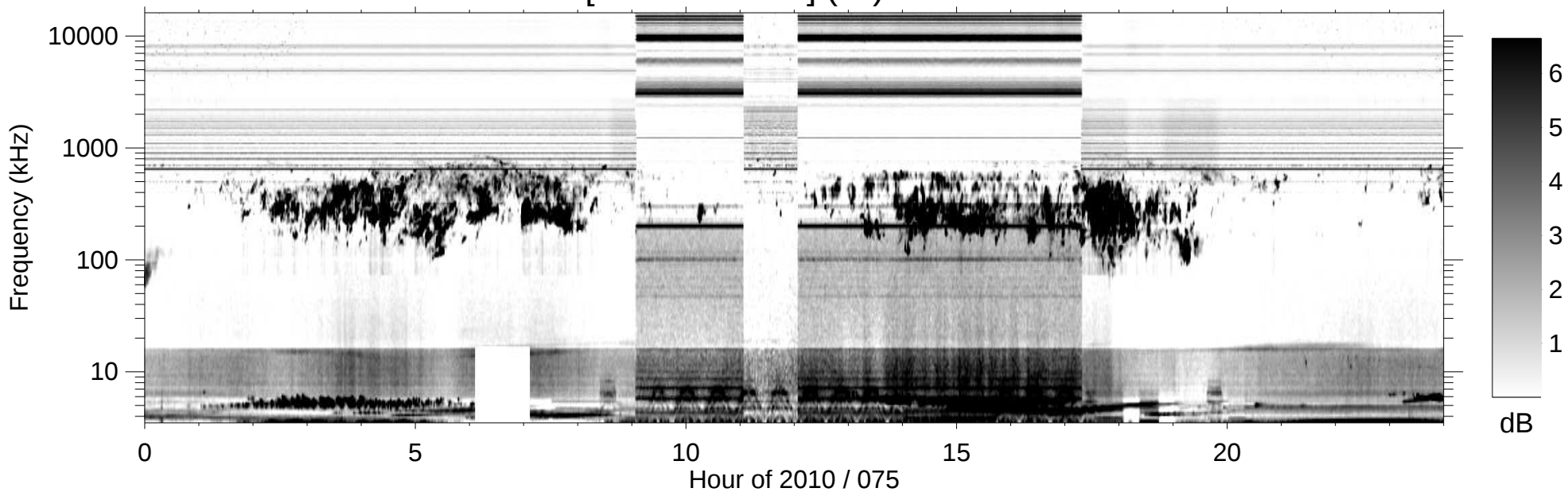
RPWS [ABCH1H2/Ex] (-B) 2010/03/16
