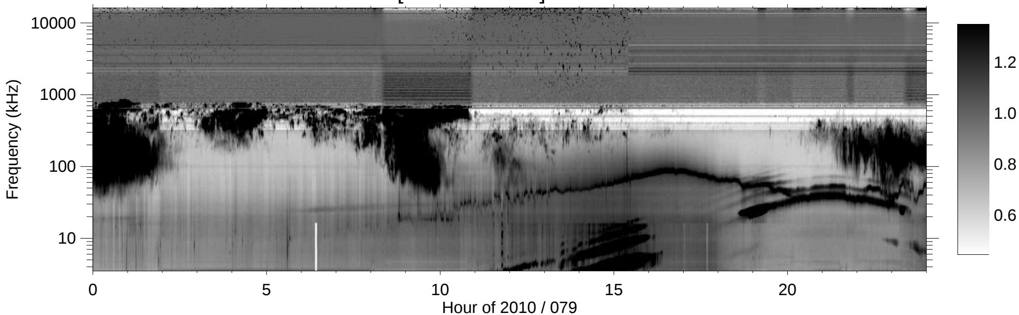
RPWS [ABCH1H2/Ex] (-B) 2010/03/20
