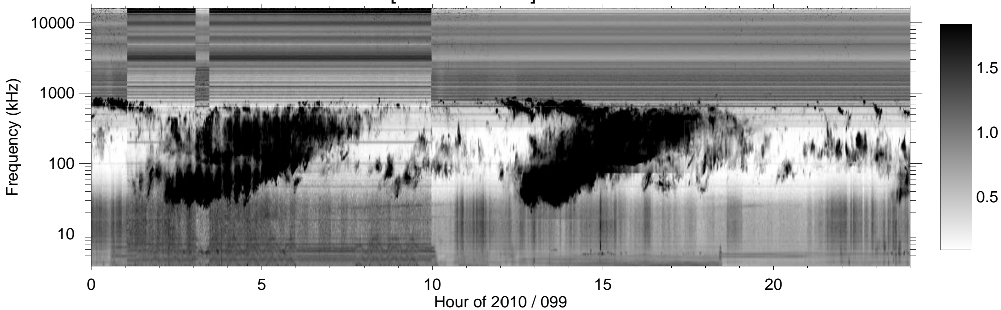
RPWS [ABCH1H2/Ex] (-B) 2010/04/09
