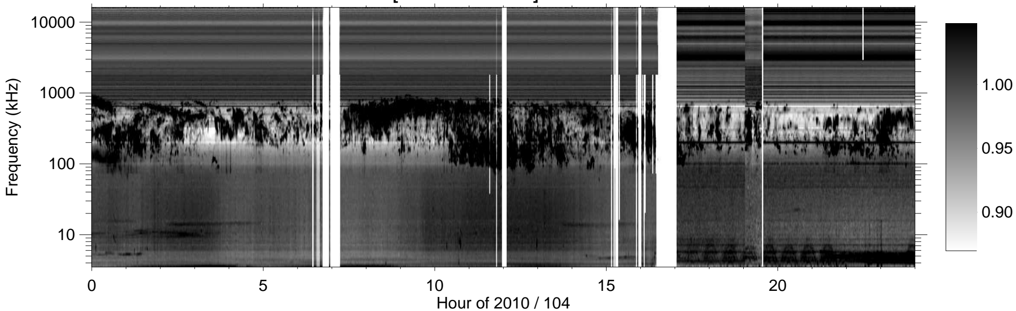
RPWS [ABCH1H2/Ex] (-B) 2010/04/14
