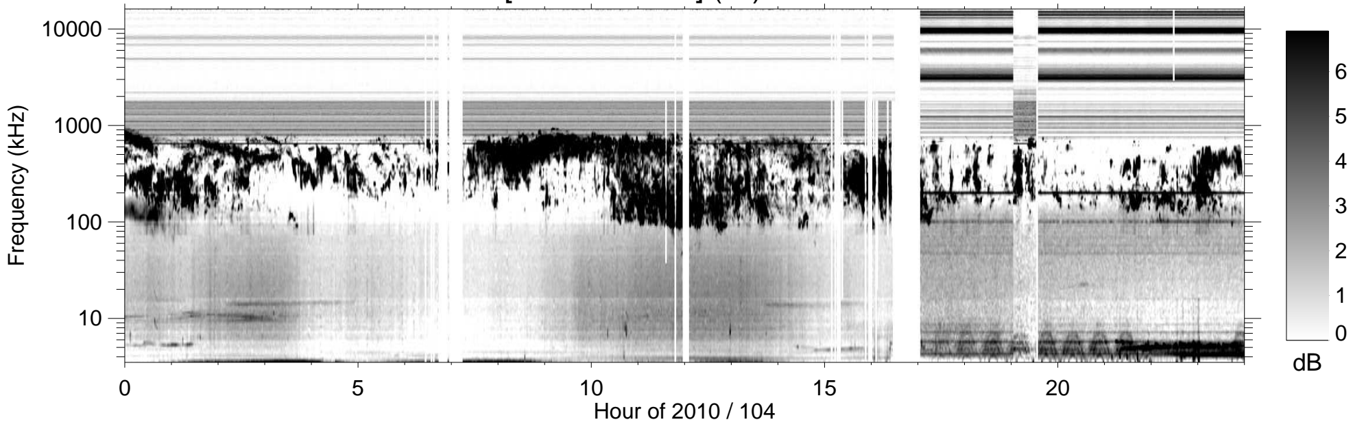
RPWS [ABCH1H2/Ex] (-B) 2010/04/14
