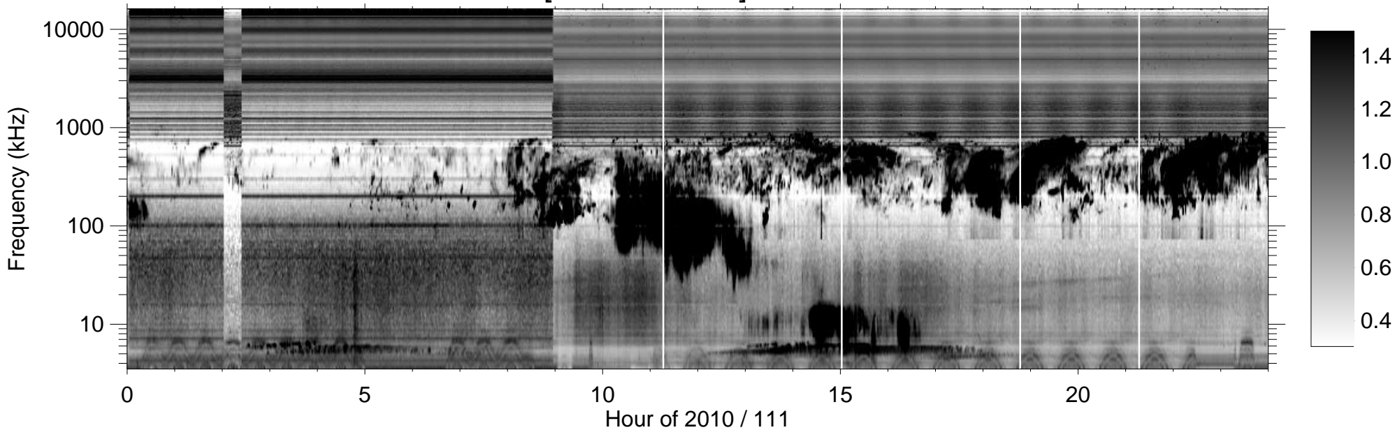
RPWS [ABCH1H2/Ex] (-B) 2010/04/21
