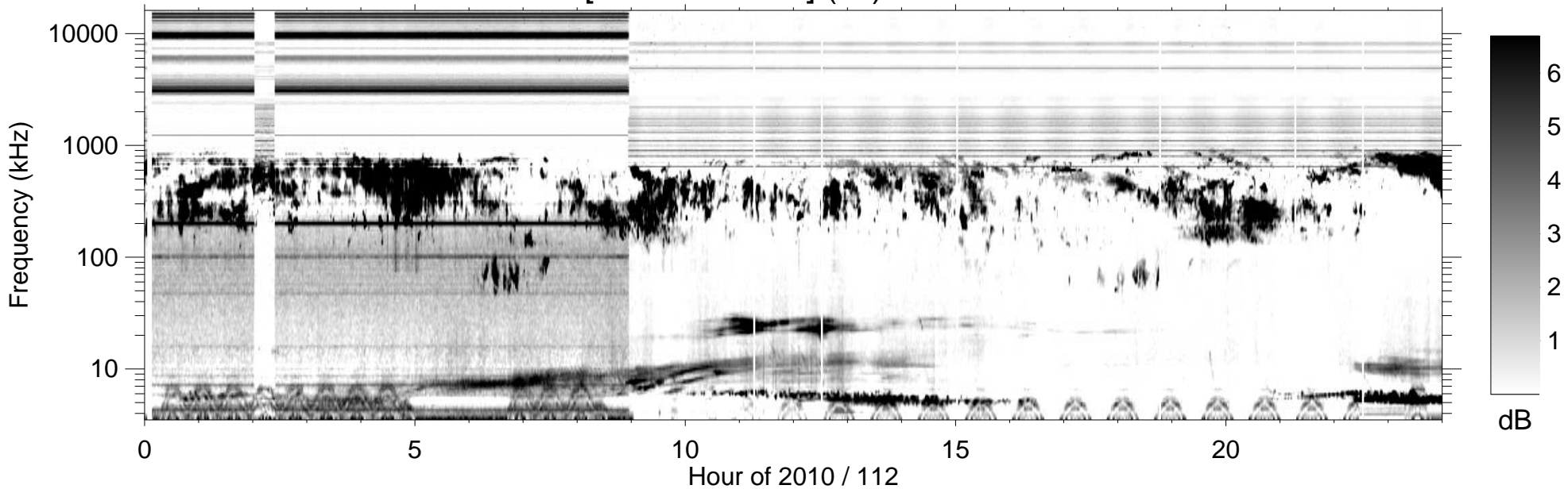
RPWS [ABCH1H2/Ex] (-B) 2010/04/22
