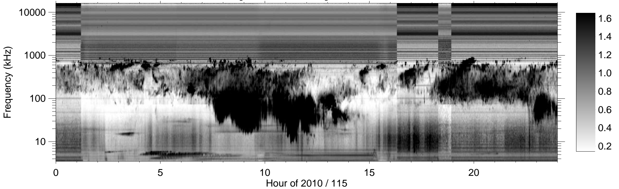
RPWS [ABCH1H2/Ex] (-B) 2010/04/25
