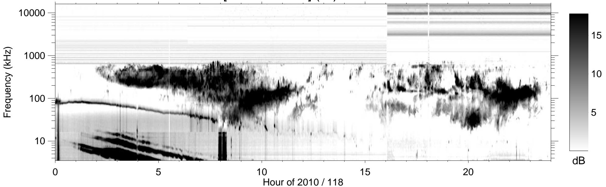
RPWS [ABCH1H2/Ex] (-B) 2010/04/28
