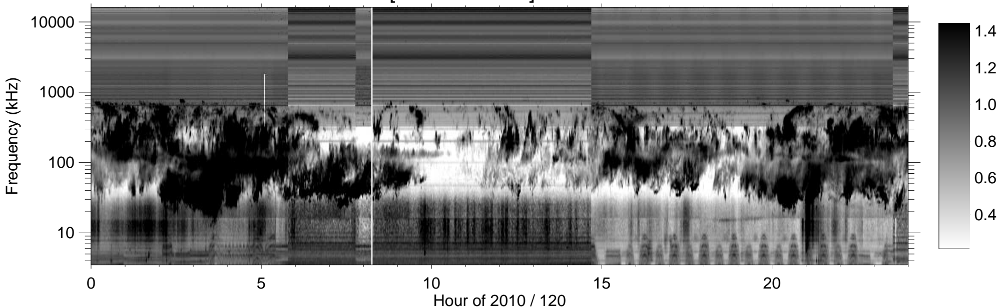
RPWS [ABCH1H2/Ex] (-B) 2010/04/30
