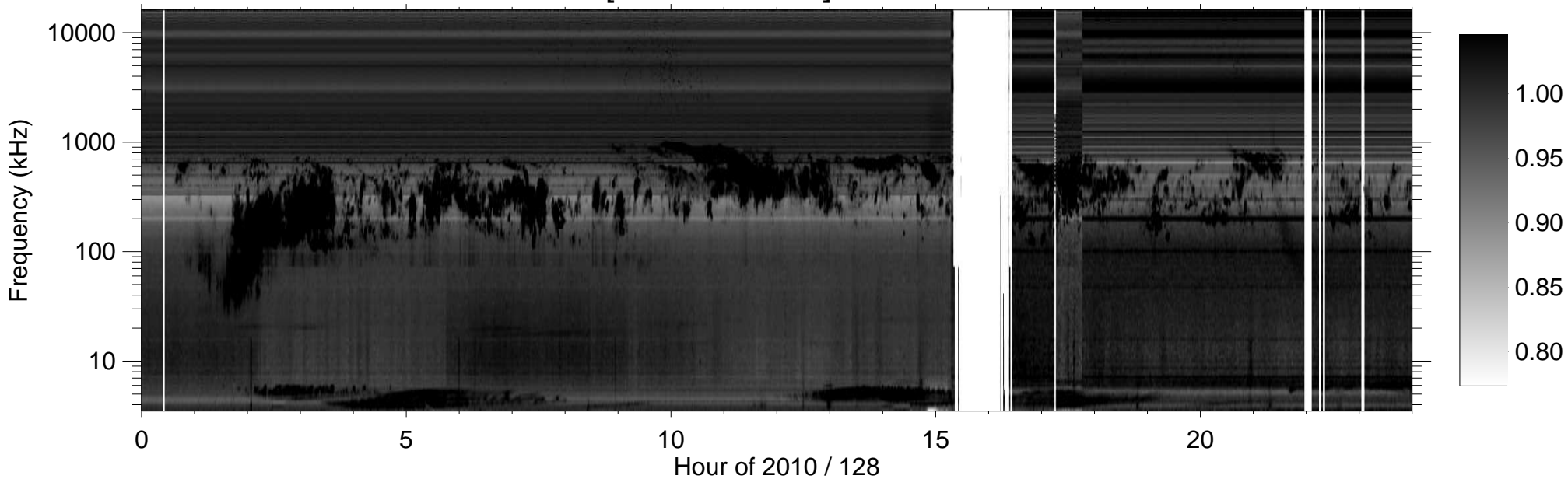
RPWS [ABCH1H2/Ex] (-B) 2010/05/08
