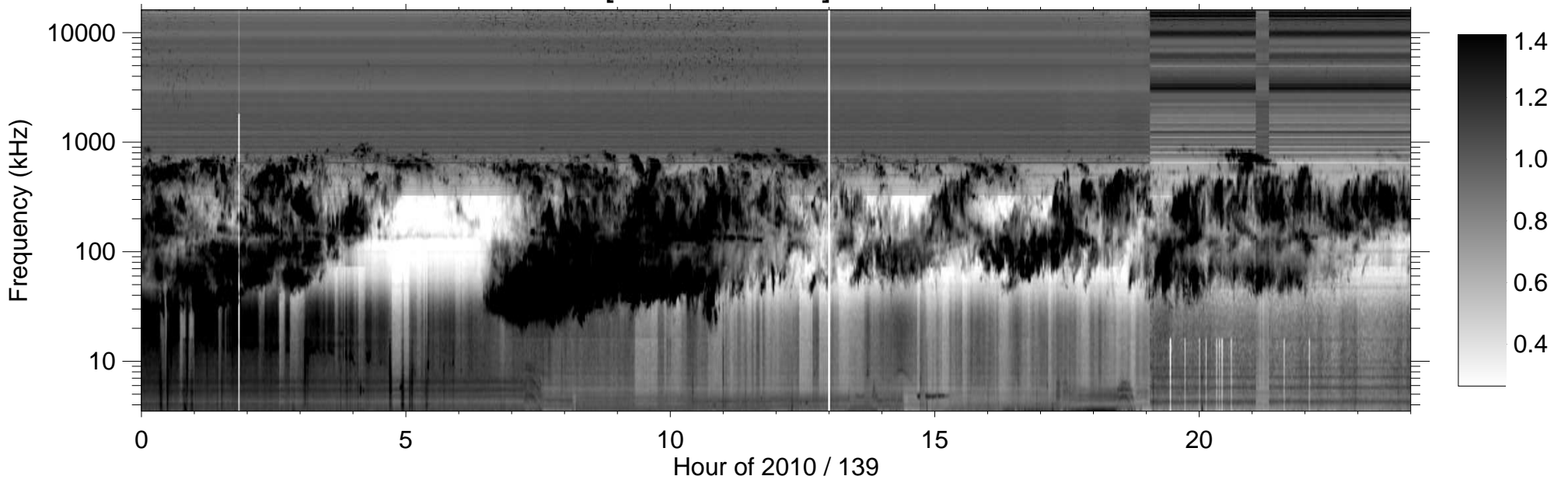
RPWS [ABCH1H2/Ex] (-B) 2010/05/19
