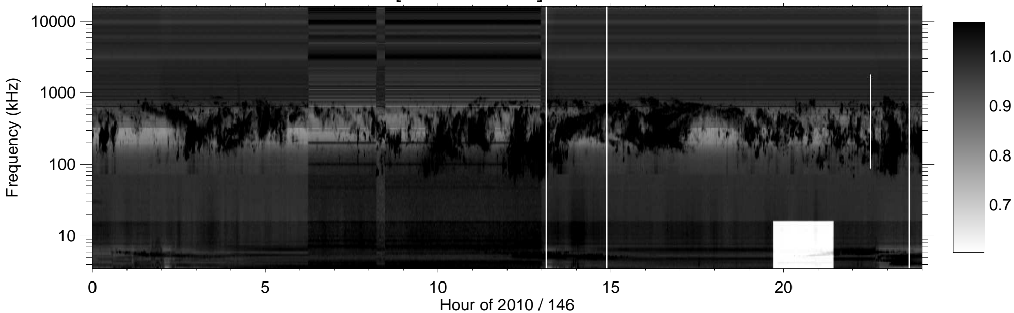
RPWS [ABCH1H2/Ex] (-B) 2010/05/26
