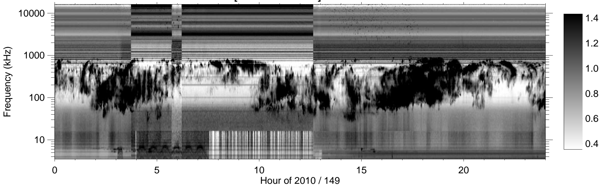
RPWS [ABCH1H2/Ex] (-B) 2010/05/29
