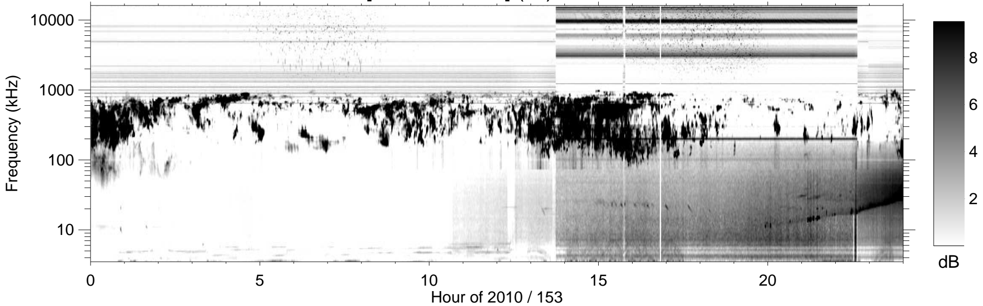
RPWS [ABCH1H2/Ex] (-B) 2010/06/02
