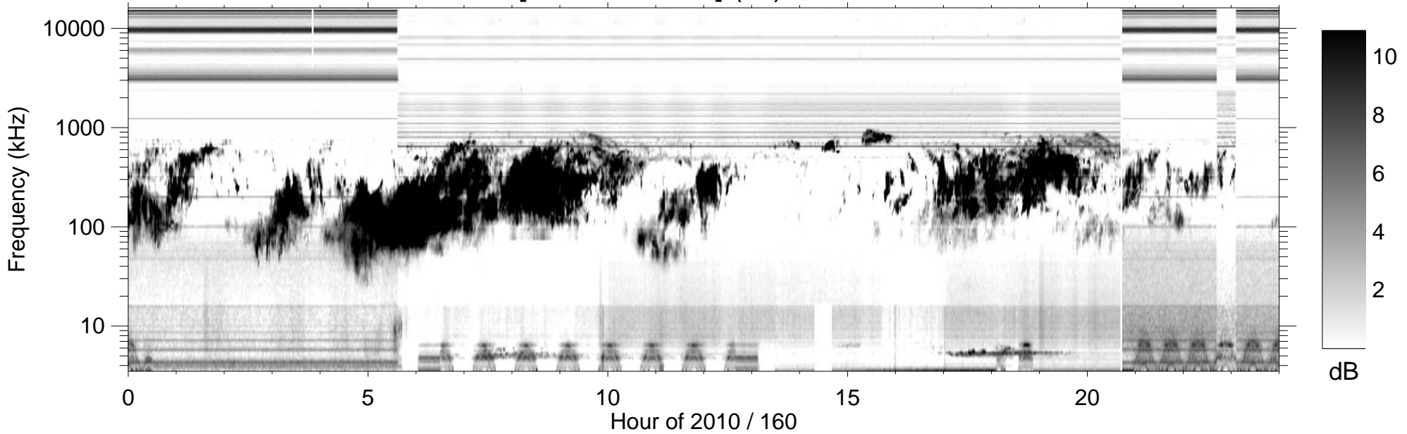
RPWS [ABCH1H2/Ex] (-B) 2010/06/09
