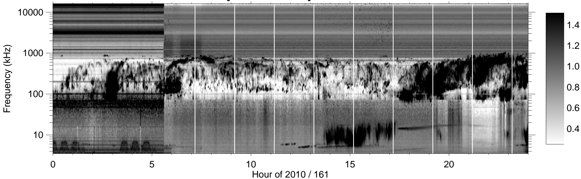
RPWS [ABCH1H2/Ex] (-B) 2010/06/10
