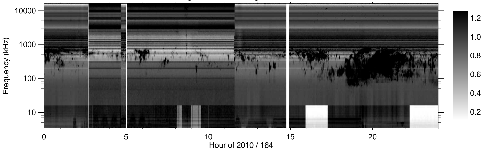
RPWS [ABCH1H2/Ex] (-B) 2010/06/13
