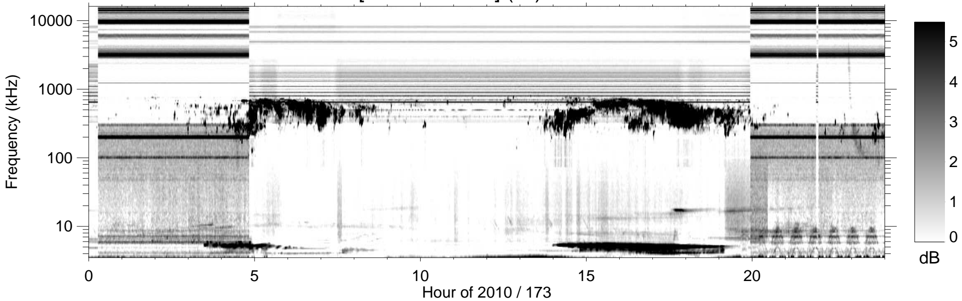
RPWS [ABCH1H2/Ex] (-B) 2010/06/22
