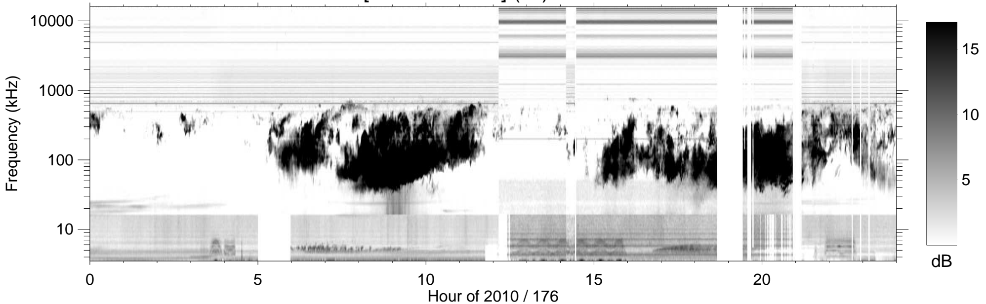
RPWS [ABCH1H2/Ex] (-B) 2010/06/25
