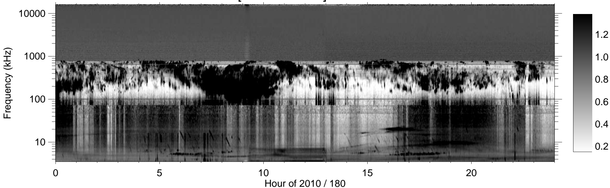
RPWS [ABCH1H2/Ex] (-B) 2010/06/29
