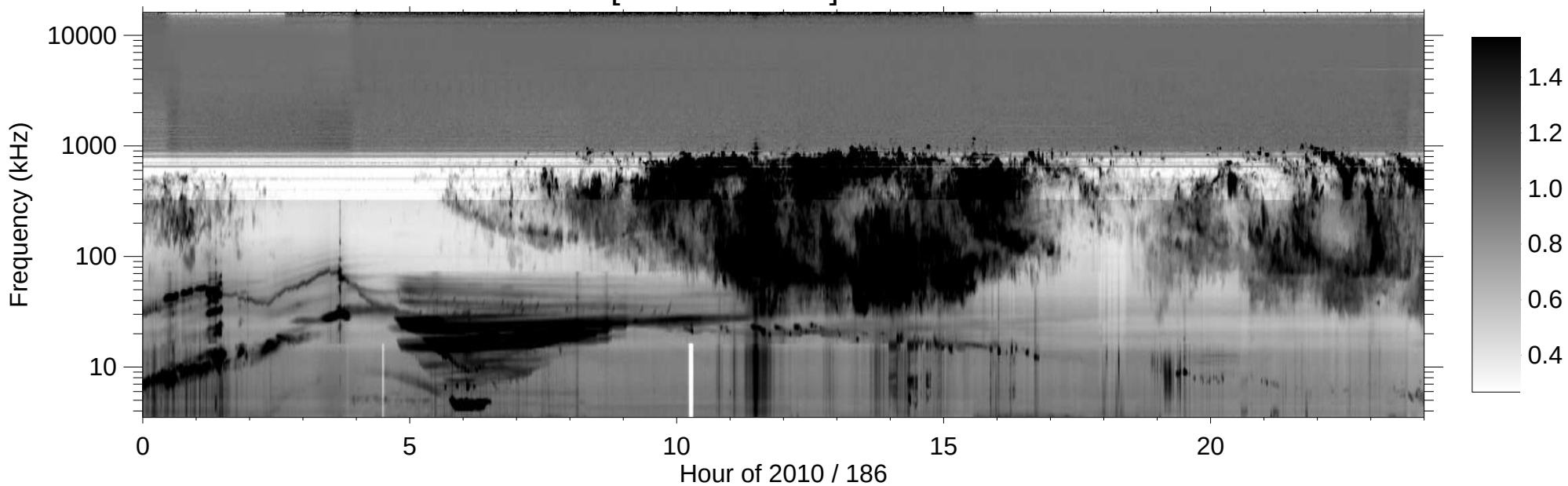
RPWS [ABCH1H2/Ex] (-B) 2010/07/05
