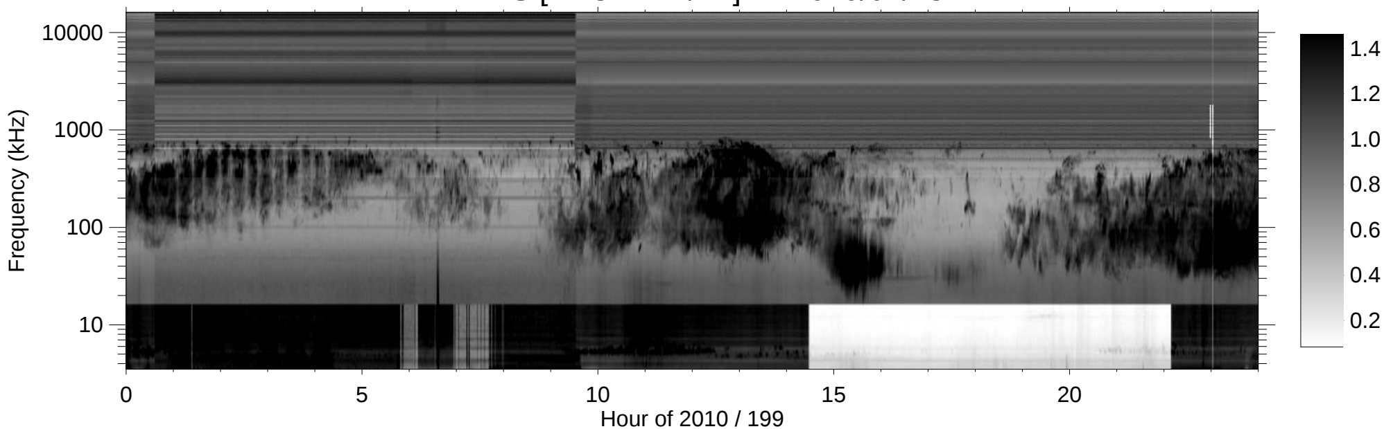
RPWS [ABCH1H2/Ex] (-B) 2010/07/18
