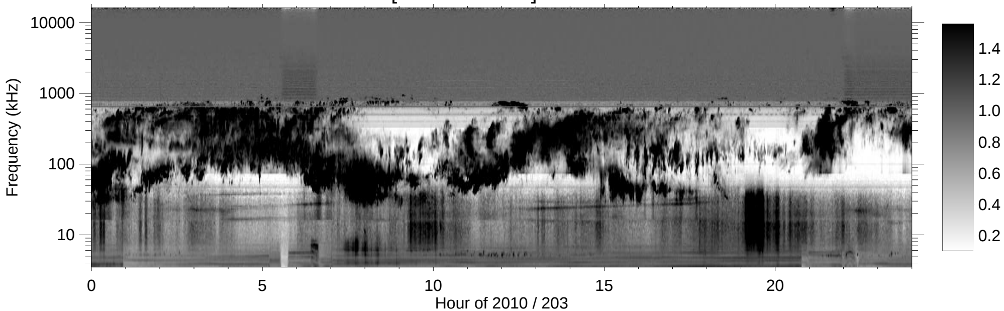
RPWS [ABCH1H2/Ex] (-B) 2010/07/22
