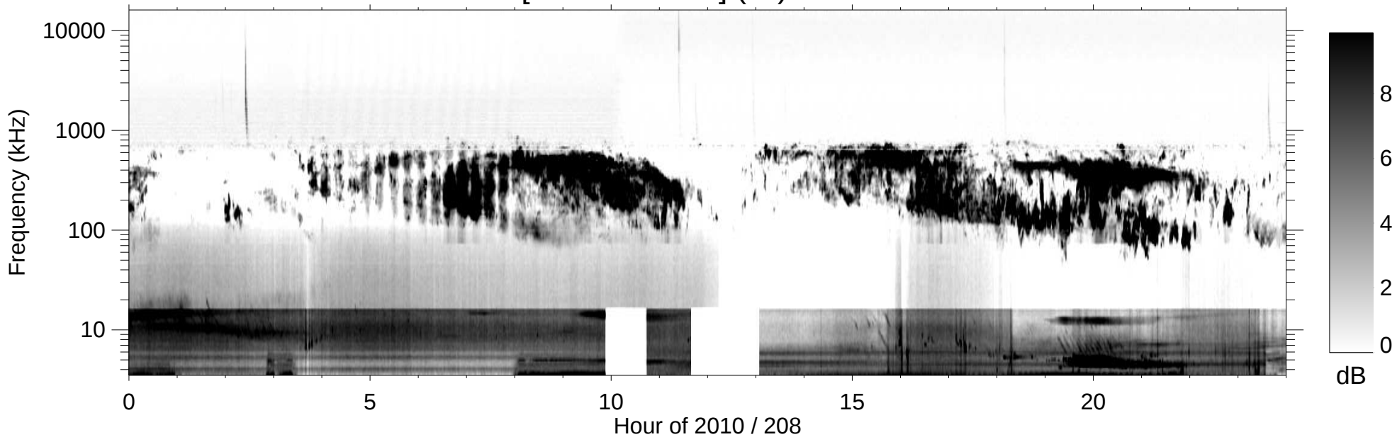
RPWS [ABCH1H2/Ex] (-B) 2010/07/27
