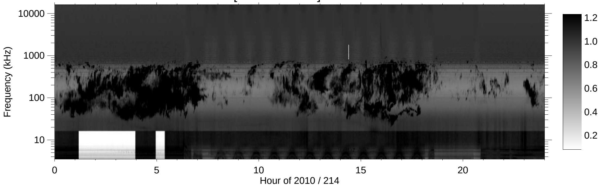
RPWS [ABCH1H2/Ex] (-B) 2010/08/02
