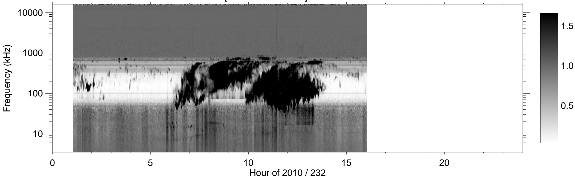
RPWS [ABCH1H2/Ex] (-B) 2010/08/20
