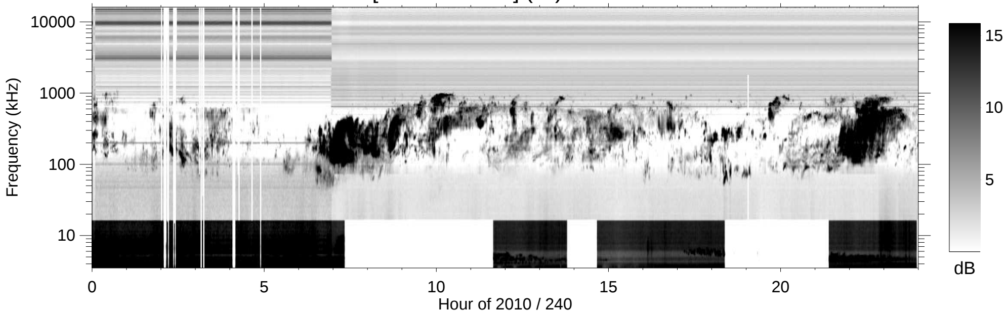
RPWS [ABCH1H2/Ex] (-B) 2010/08/28
