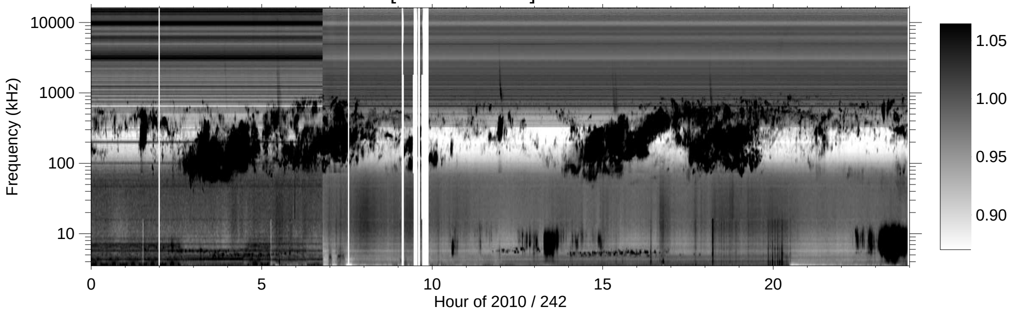
RPWS [ABCH1H2/Ex] (-B) 2010/08/30
