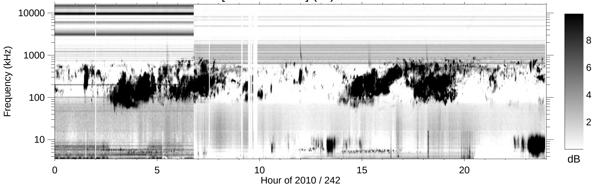
RPWS [ABCH1H2/Ex] (-B) 2010/08/30
