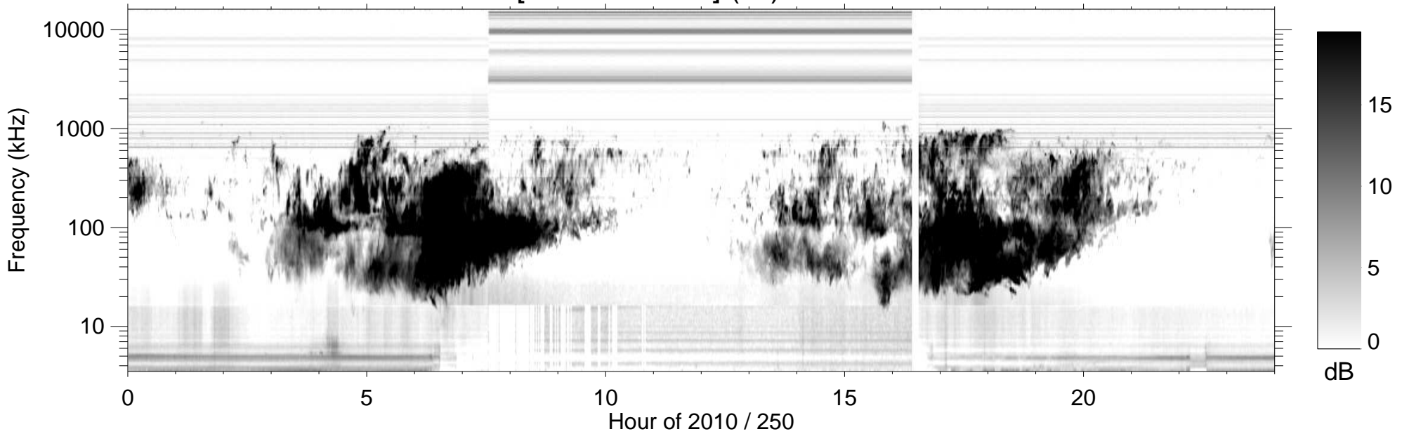
RPWS [ABCH1H2/Ex] (-B) 2010/09/07
