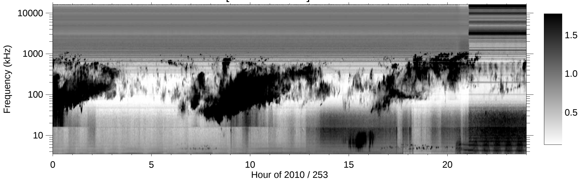
RPWS [ABCH1H2/Ex] (-B) 2010/09/10
