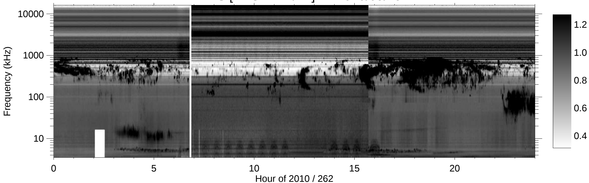
RPWS [ABCH1H2/Ex] (-B) 2010/09/19
