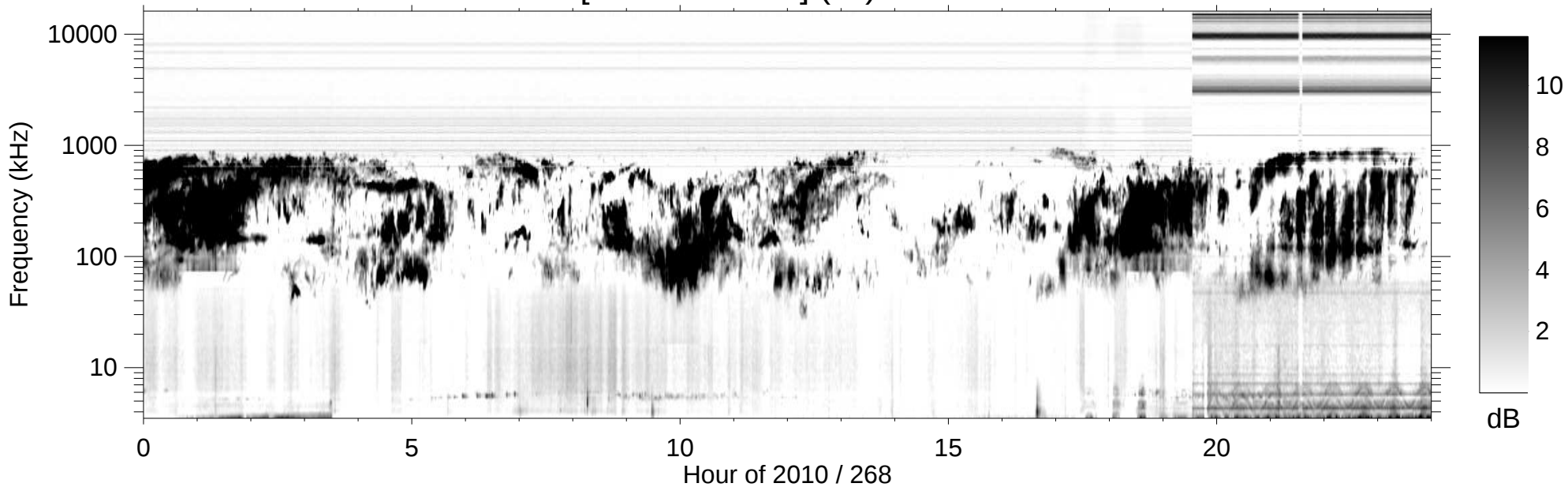
RPWS [ABCH1H2/Ex] (-B) 2010/09/25
