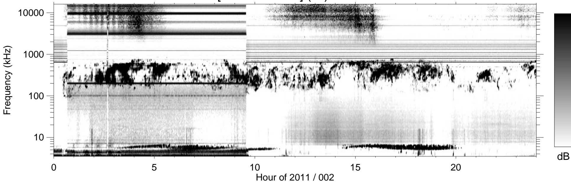
RPWS [ABCH1H2/Ex] (-B) 2011/01/02
