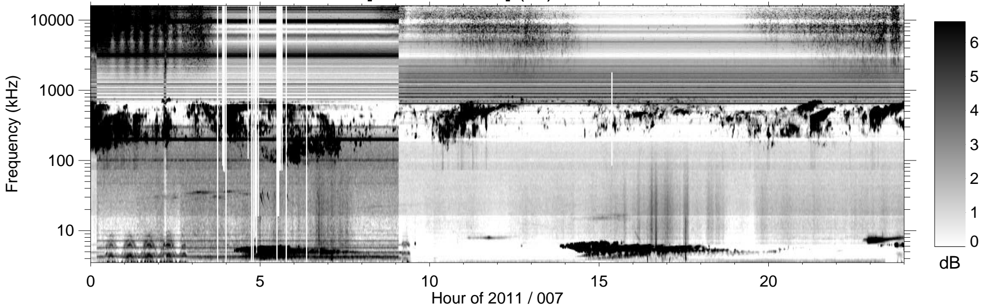
RPWS [ABCH1H2/Ex] (-B) 2011/01/07
