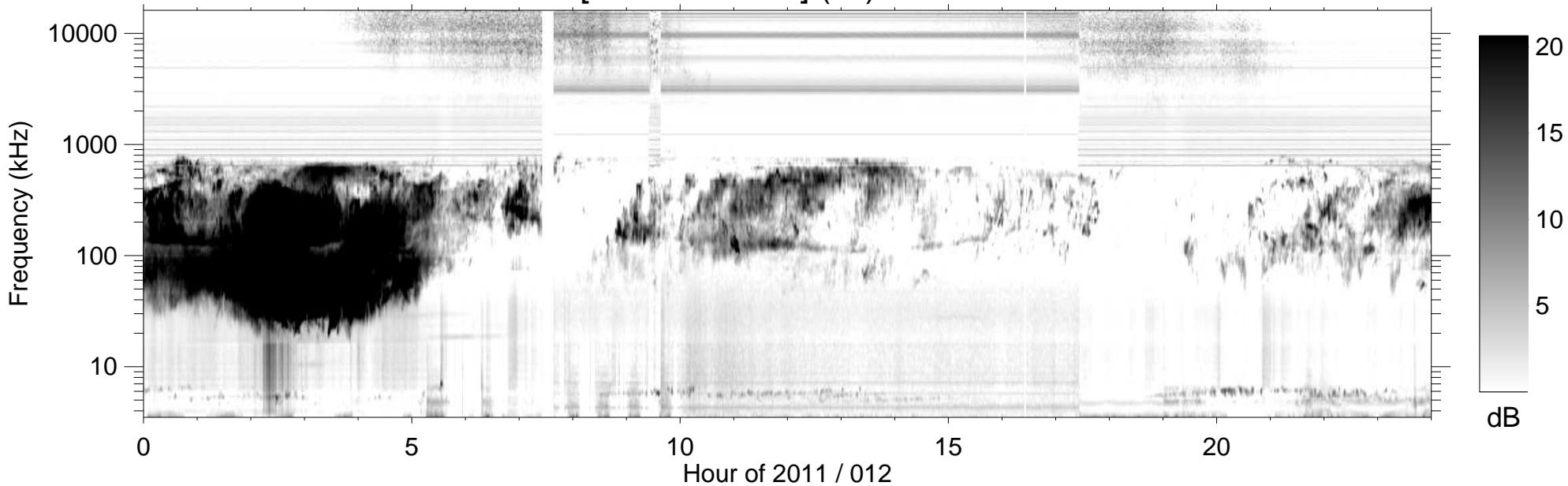
RPWS [ABCH1H2/Ex] (-B) 2011/01/12
