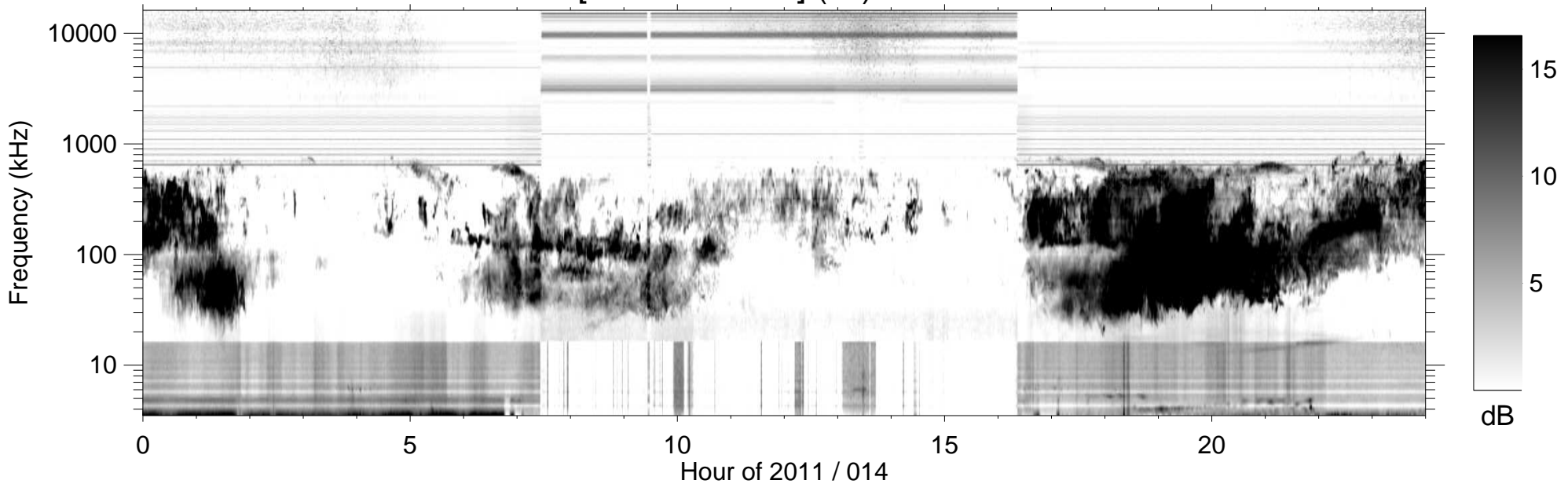
RPWS [ABCH1H2/Ex] (-B) 2011/01/14
