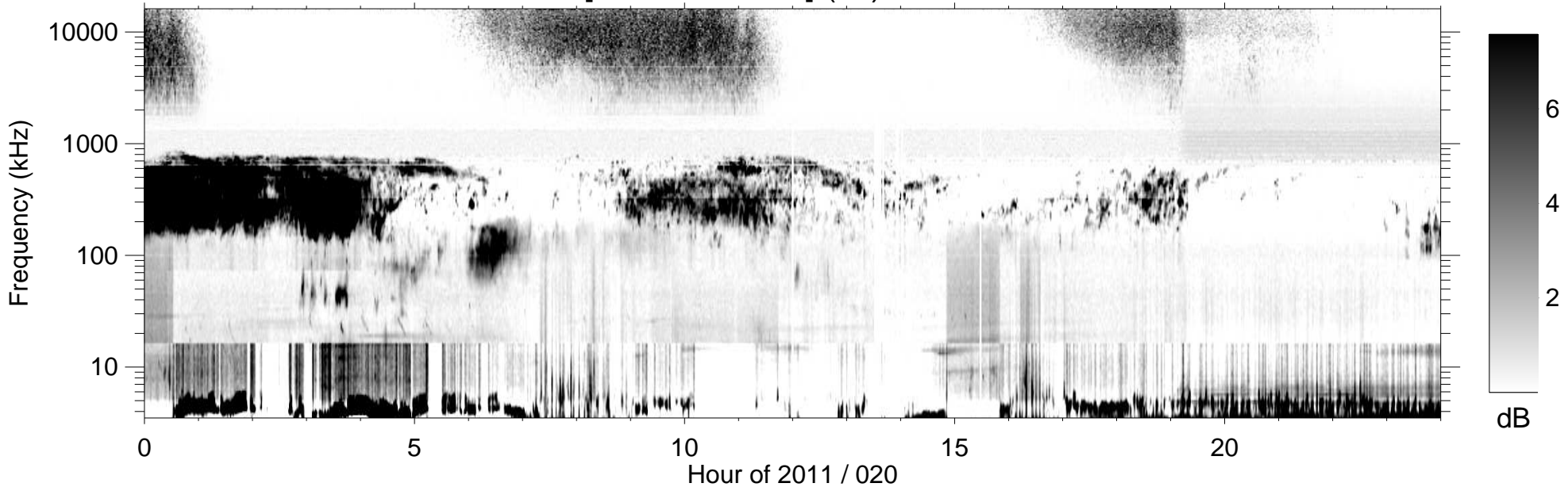
RPWS [ABCH1H2/Ex] (-B) 2011/01/20
